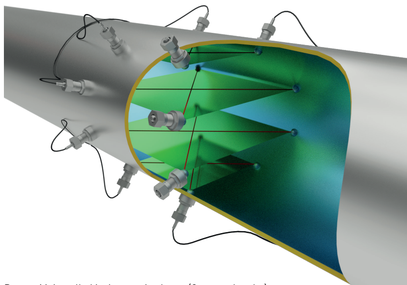
Ductus M, installed in 4 acoustic planes (8 crossed paths)
